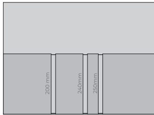
Depths can be adjusted on-site by cuttend to the required length. With grooves for cutting to length at the construction site.
